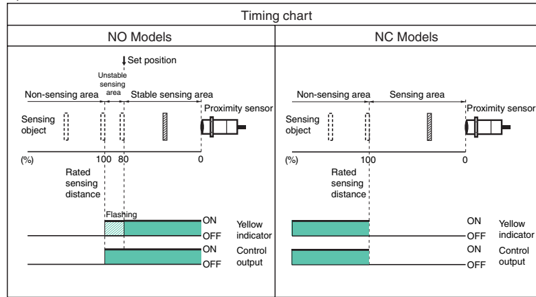
Operation mode
